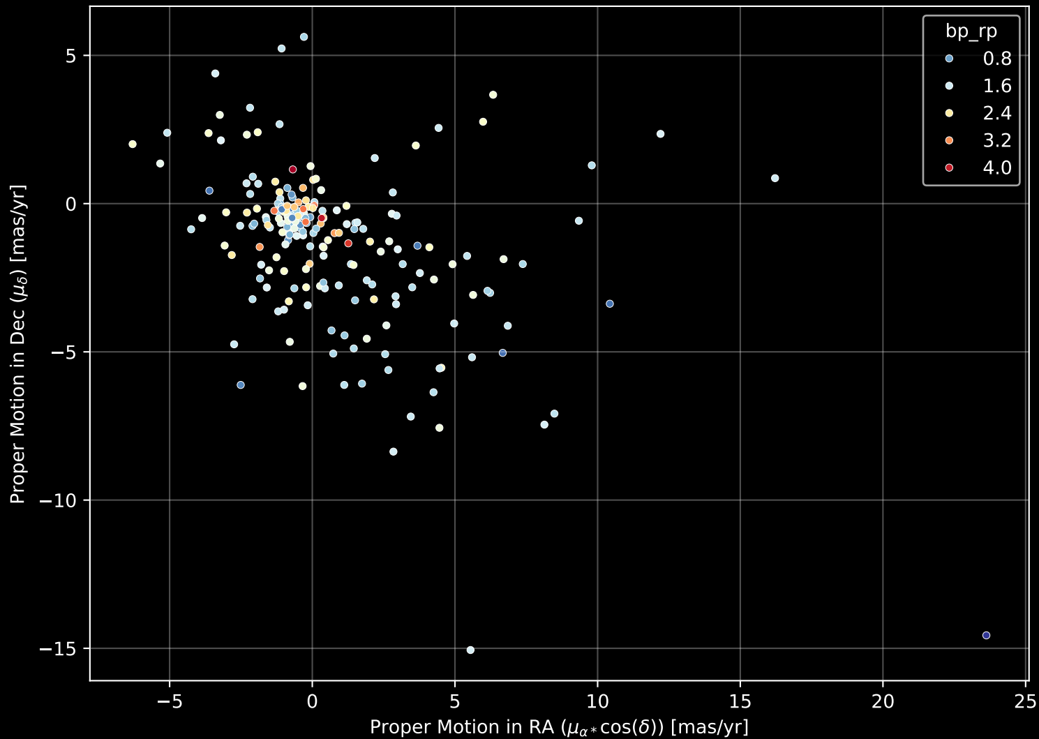
APOGEE DR17 Field: [W34_btx] Proper Motion Diagram (n= 213)
