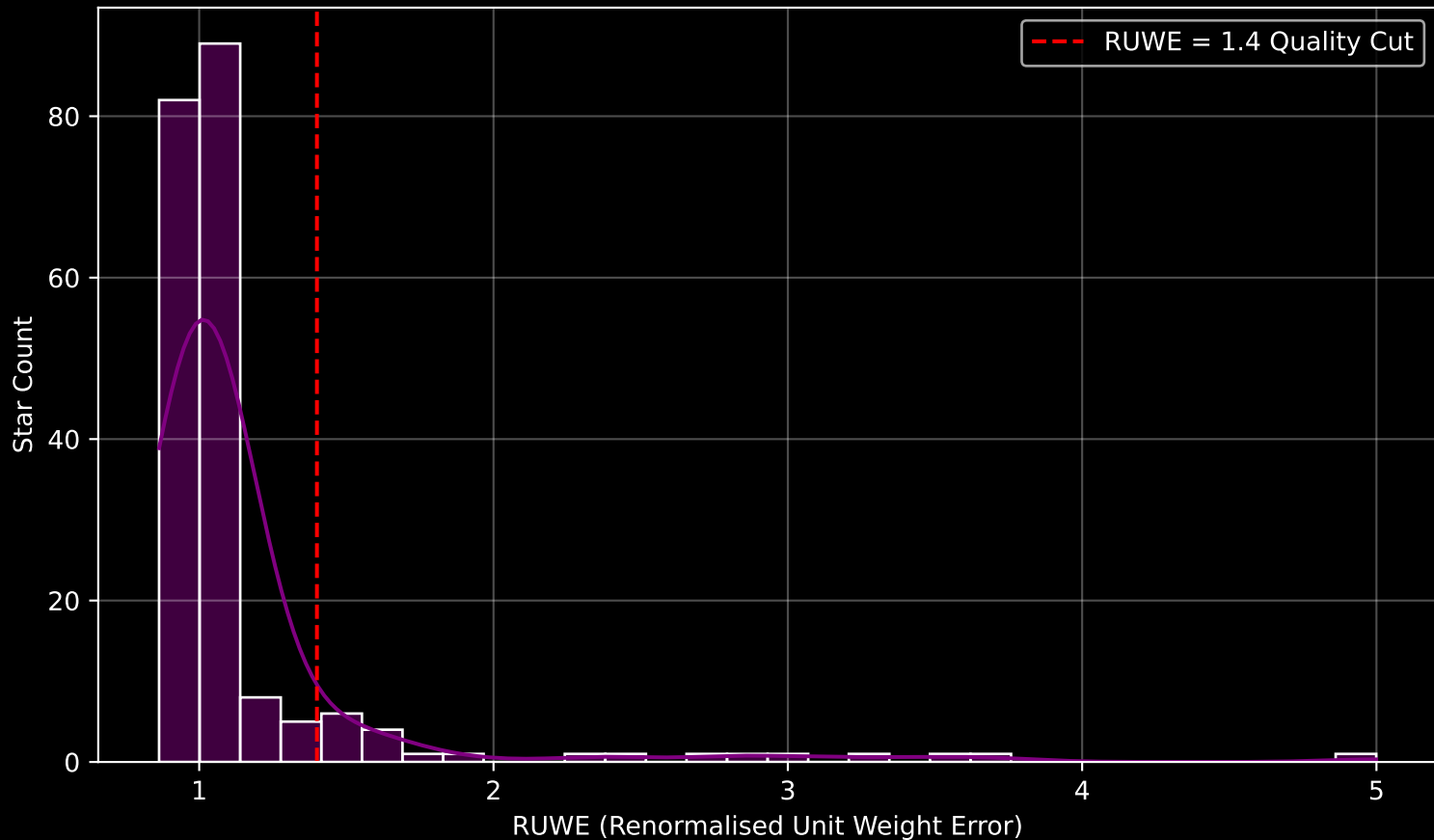
GAPOGEE DR17 Field [W34_btx] RUWE Distribution (n= 205)
