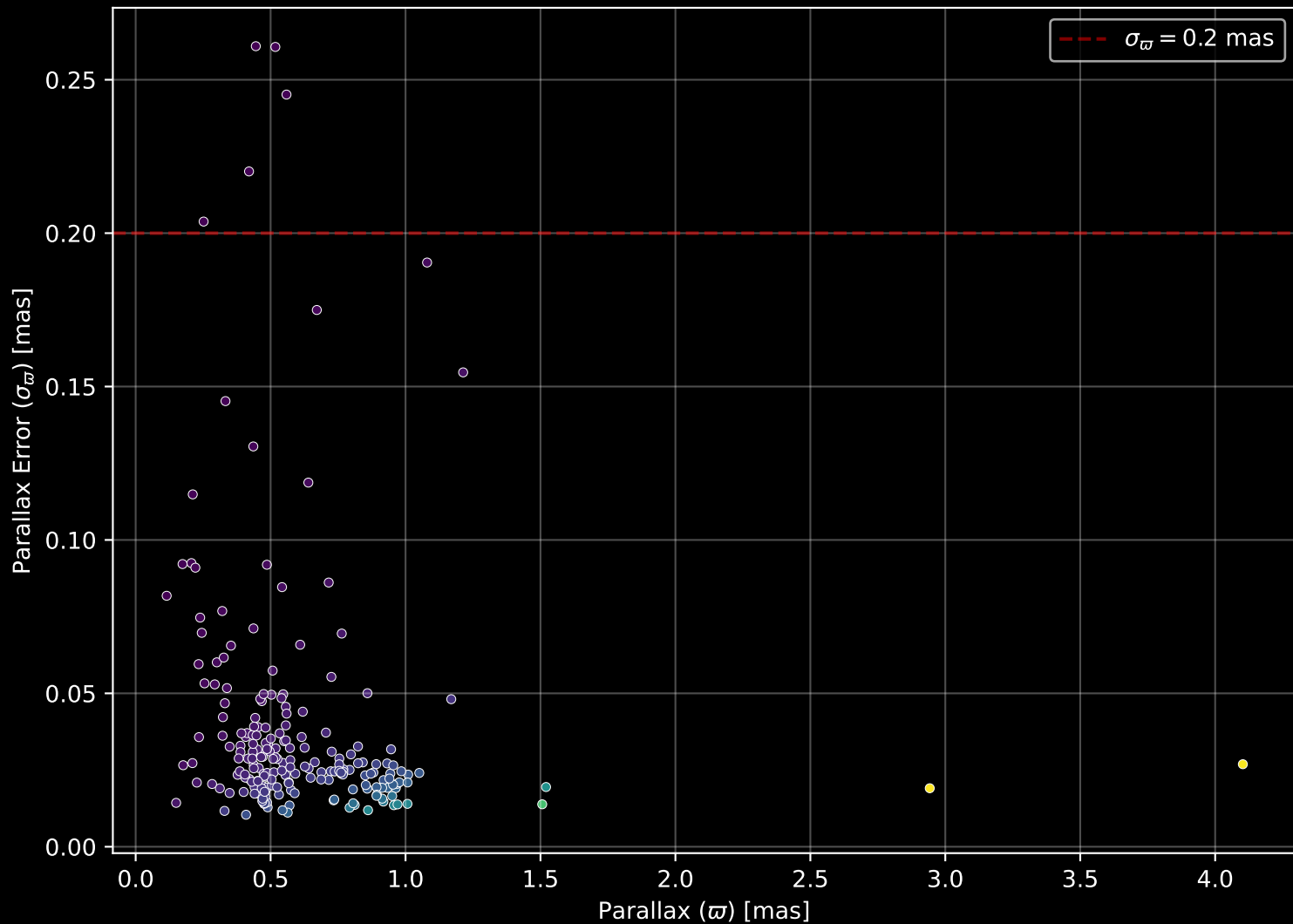
APOGEE DR17 Field: [W34_btx] Parallax Quality (n= 213)
