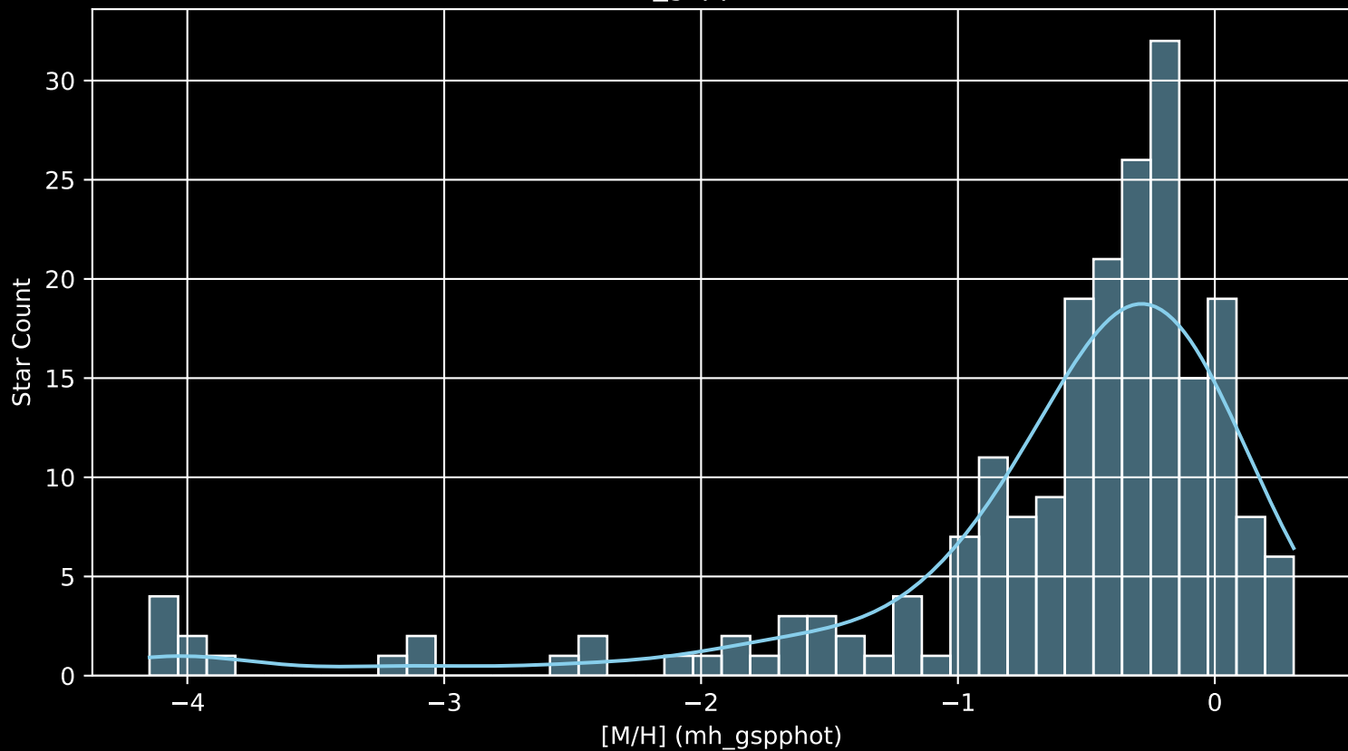
APOGEE DR17 Field: [W34_btx [M/H] (mh_gspphot) (n= 213)
