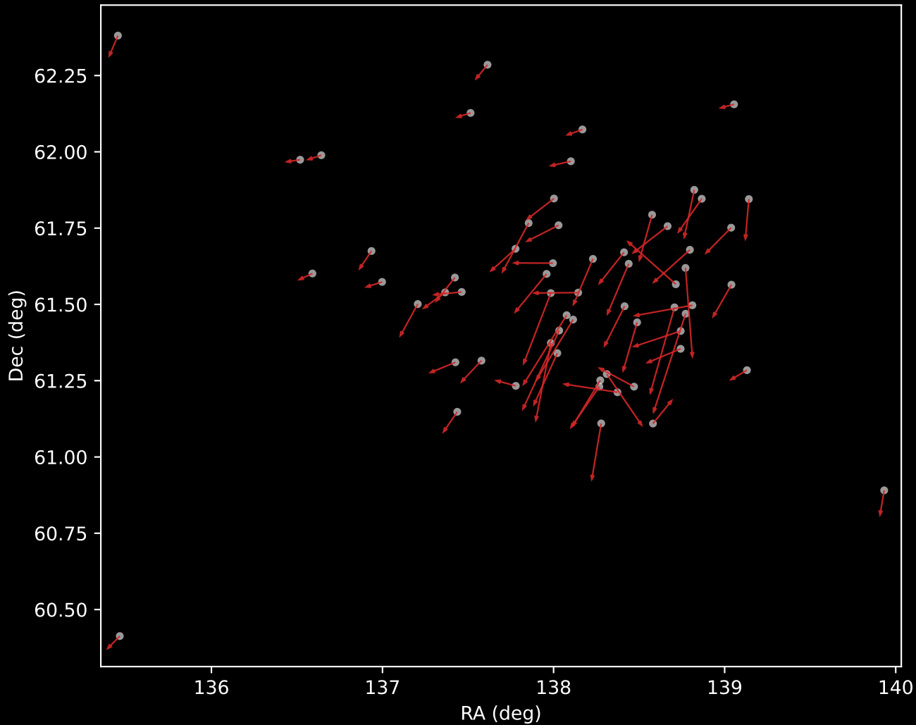
APOGEE DR17 Cluster 6 Proper Motion Vectors (n=62)
